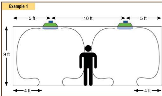
Figure 7 (left): Diffuser Performance. Two louver-faced 15 in. × 15 in. (381 mm × 381 mm) inlets. Each diffuser is 469 cfm (1650 L/s), totaling 938 cfm. Throw data is 18 (50 fpm) and NC < 20 . Use the T_{50}/L ratio to obtain ADPI range for 90%: 1.4 to 2.7 and T_{50}/L calculation 18/5 = 3.6 . Figure 8 (right): Diffuser Performance. One louver-faced 21 in. × 21 in. inlets with four-way discharge. Each diffuser is 919 cfm. Throw data is 24 (50 fpm) and NC < 20 . Use the T_{50}/L ratio to obtain ADPI range for 90%: 1.4 to 2.7 and T_{50}/L calculation 24/10 = 2.4 .
