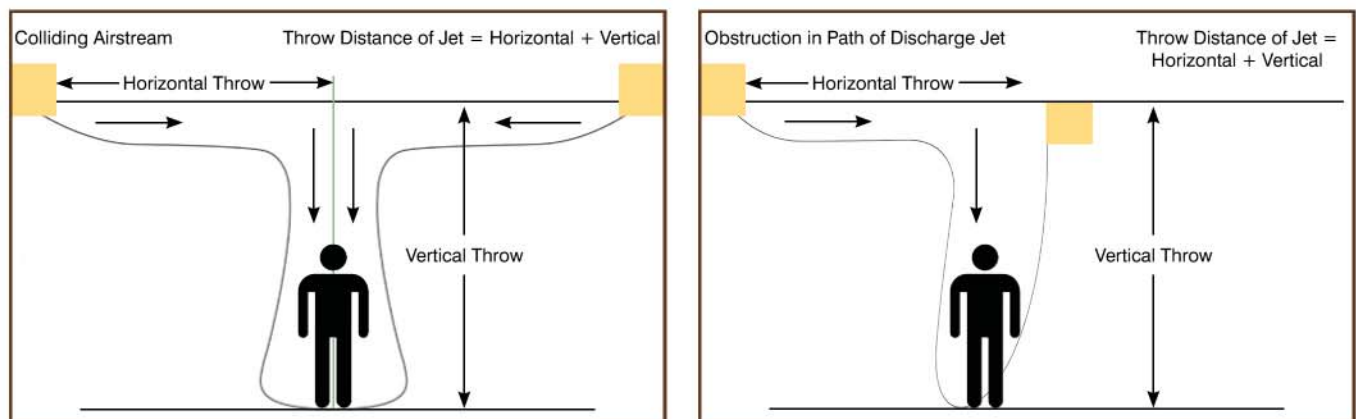
Figure 5 (left): Colliding airstreams can project a high velocity airstream into the occupied zone. This can be predicted by mapping the catalog throw data or the T_{50}/L ratio. Figure 6 (right): Obstructions in the airstream such as architectural details and support beams can force the supply jet down into the occupied zone causing occupant discomfort.
